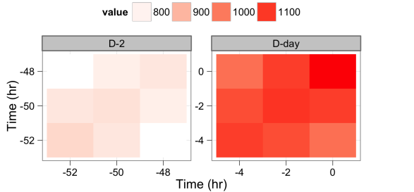
Fig. 7. Temporal covariance matrices: \Sigma_{\text{normal}} and \Sigma_{\text{risky}} .
